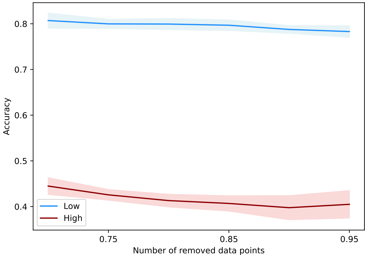
DataAttrOpt(10000, 0.1, 15, best, +b, alpha=best) - imdb-embeddings
